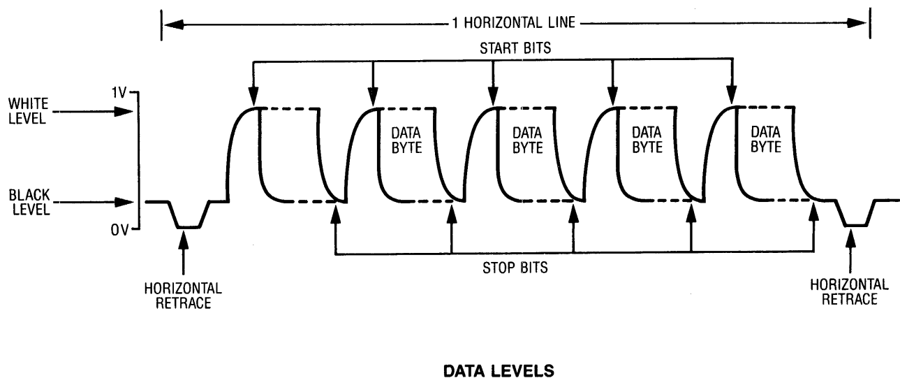
Figure 3. Video Signal
