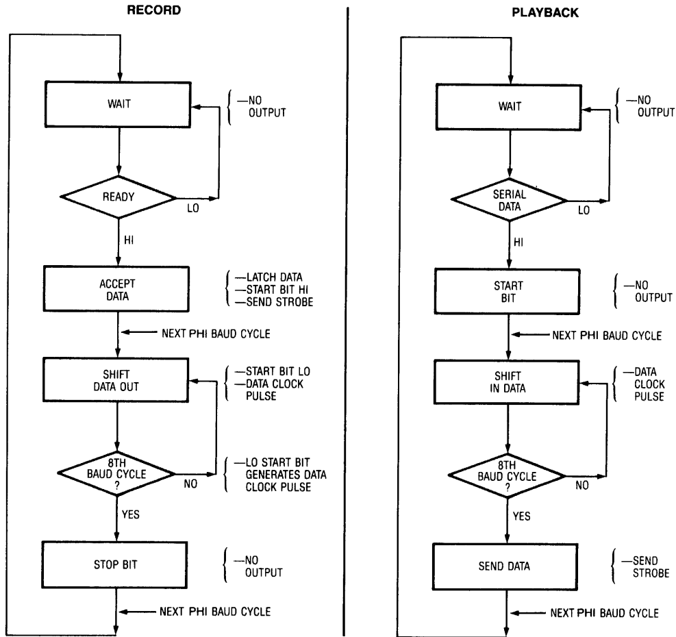
Figure 5. Control State Machine
