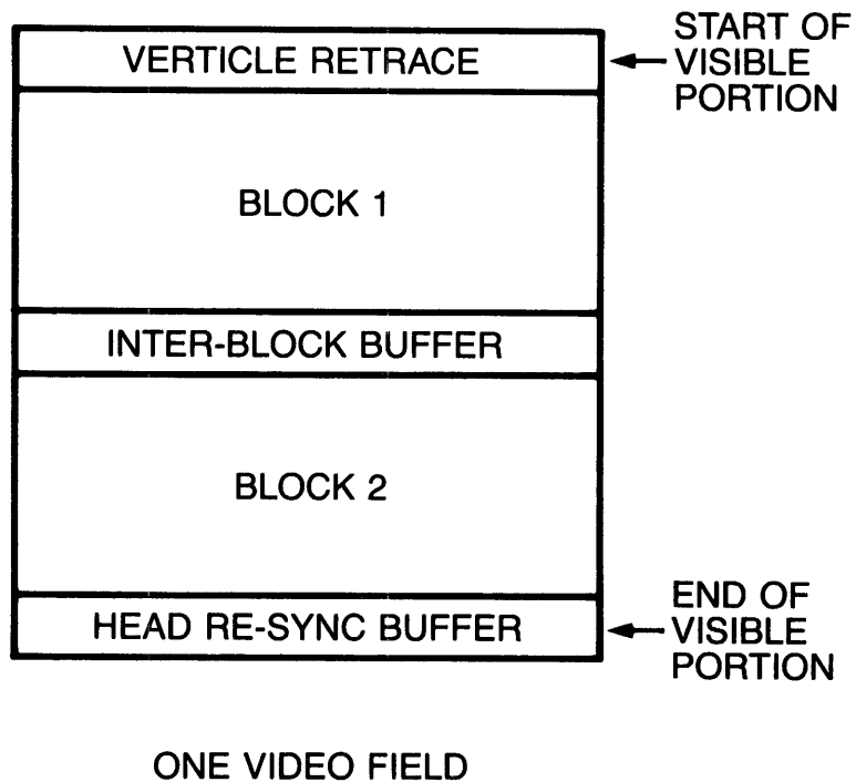
Figure 1. Video Frame
