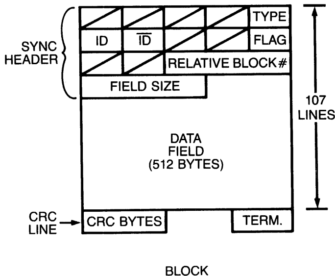
BLOCK Figure 2. Video Format
